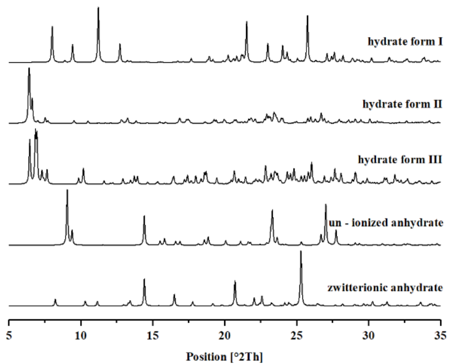
Figure S2. X-ray diffractograms of CIP polymorphs from Cambridge Crystallographic Data Centre
