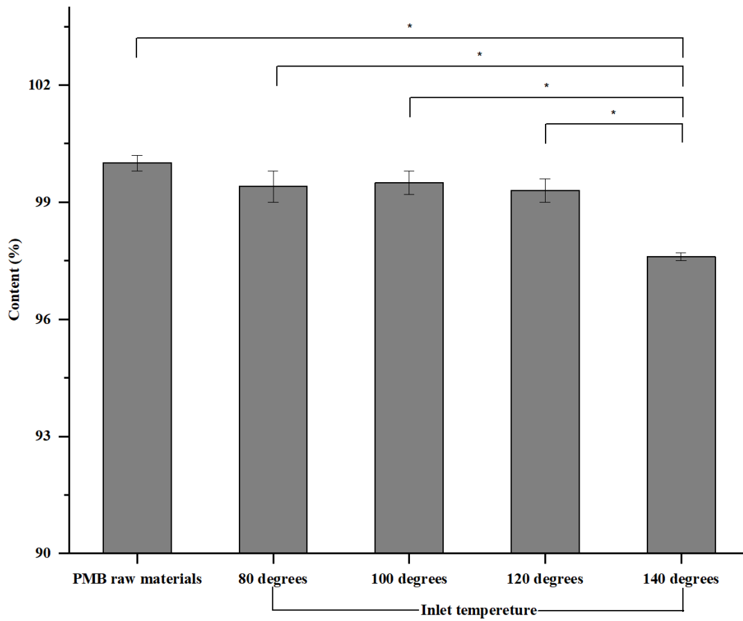
Figure S1. Mass content (%) of PMB spray dried powders at different inlet temperature
